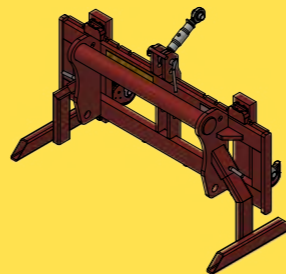
Adaptor Maniscopic - Three point hitch Cat. 2
